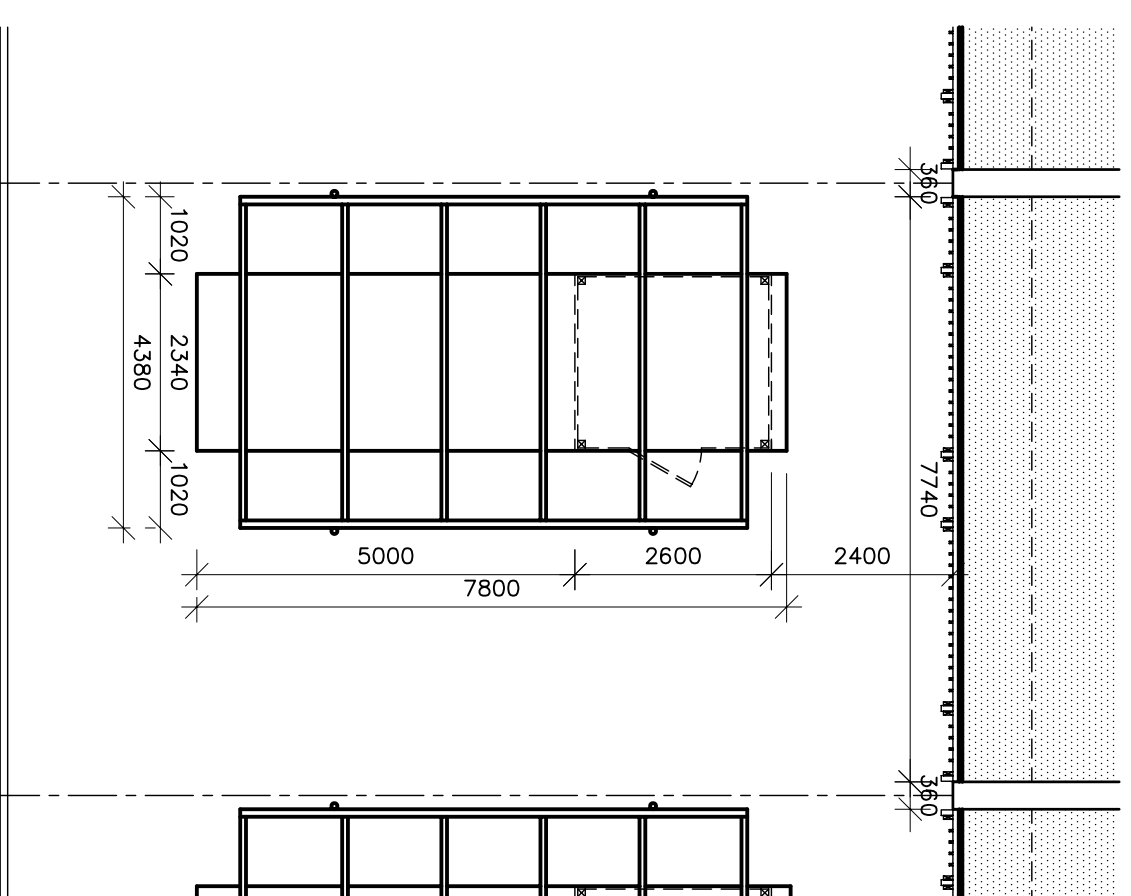
Situationsplan, 1:100
